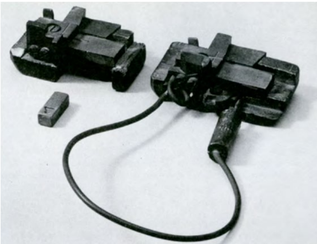
Fig. 11, 12 Typecasting mould, ladle and matrix. From the Berling collection, Kulturen.
