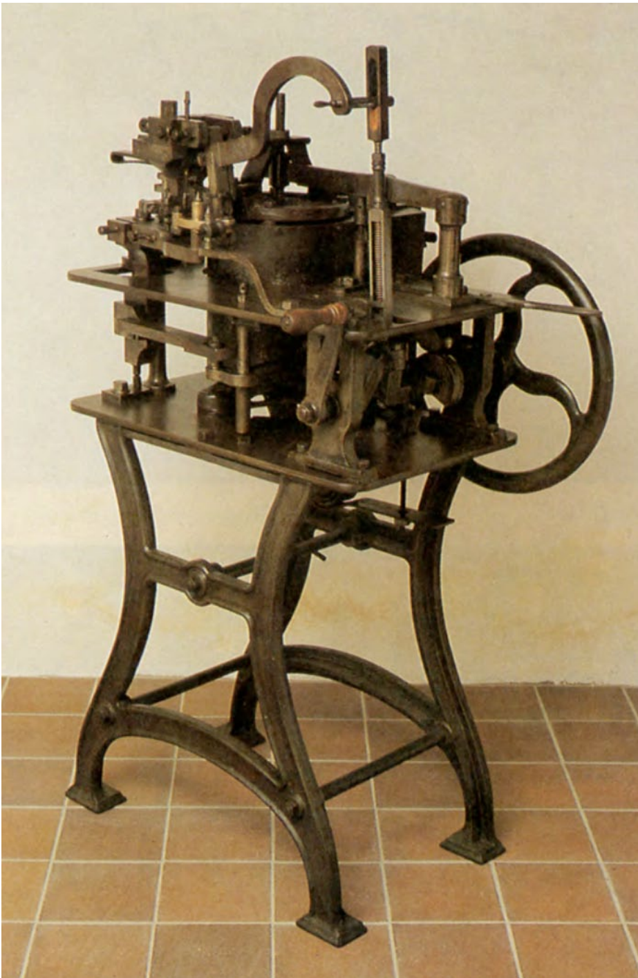
Fig. 9 Pivotal typecasting machine in the Berling collection, Kulturen.
