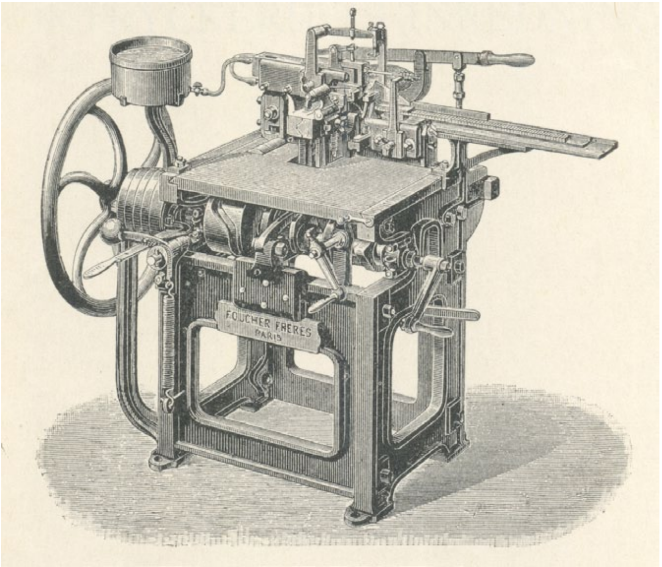
Fig. 10 'Automatic' typesetting machine. (Elge, 1915)
